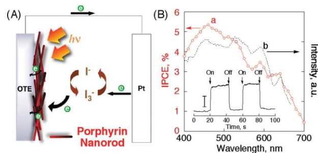
Fig. 3 (A) An illustration of the photoelectrochemical solar cell. (B) (a) Photocurrent (IPCE) action spectrum of \text{H}_2\text{DBuPP} nanorod on an OTE. Electrolyte: 0.5 mol \text{dm}^{-3} LiI and 0.01 mol \text{dm}^{-3} \text{I}_2 in acetonitrile. (b) Excitation spectrum of \text{H}_2\text{DBuPP} nanorod on an OTE; observed at 710 nm. The insertion shows photocurrent generation responses under white light illumination using an AM 1.5 filter. Input Power: 42 mW \text{cm}^{-2} . The bar is 50 \mu\text{A cm}^{-2} .
