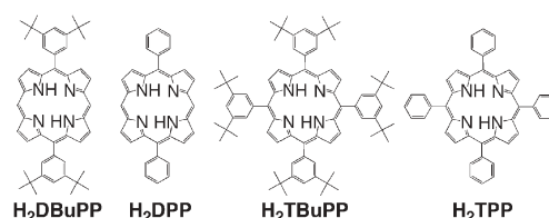
Chart 1 Porphyrin compounds bearing different substituents at meso -positions in this study.
