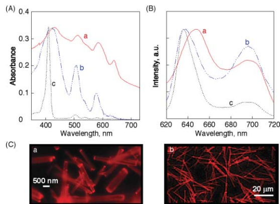
Fig. 2 (A) Absorption and (B) fluorescence spectra of (a) \text{H}_2\text{DBuPP} nanorod film, (b) \text{H}_2\text{DBuPP} drop-cast film on quartz plates and (c) \text{H}_2\text{DBuPP} ( 4 \times 10^{-6} mol \text{dm}^{-3} ) in toluene. The excitation wavelength is 410 nm. (C) Fluorescence images of (a) \text{H}_2\text{DBuPP} nanorod and (b) \text{H}_2\text{DBuPP} fiber.
